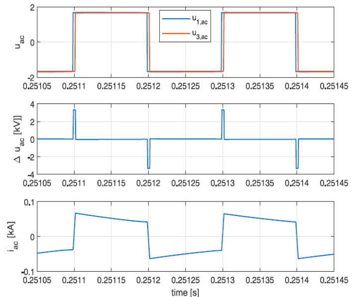
Figure 5: Bipolar switching MAB operation; input voltage to the winding 1 and 3 of the MAB (top), the corresponding differential voltage on the leakage inductance (middle) and the resulting current on winding 1 (bottom).
